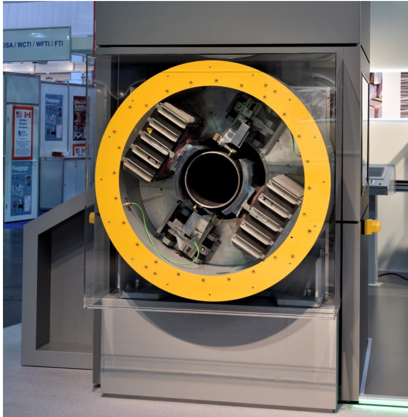
Figure 3: Presentation of the innovative ROTOMAT DA for tube testing
